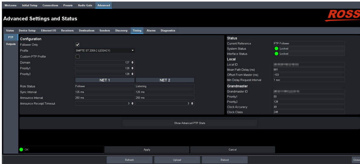
Figure 37 Example of the Advanced > Timing > PTP Tab
