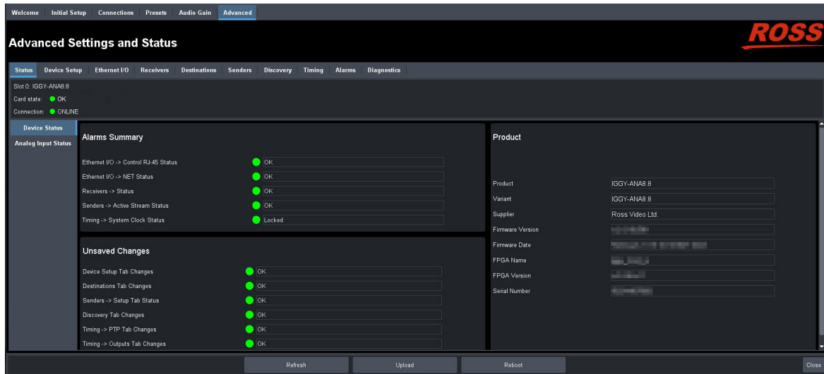
Figure 30 Example of the Advanced > Status > Device Status Tab
