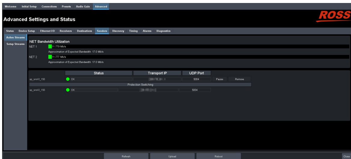
Figure 35 Example of the Advanced > Senders > Active Streams Tab
